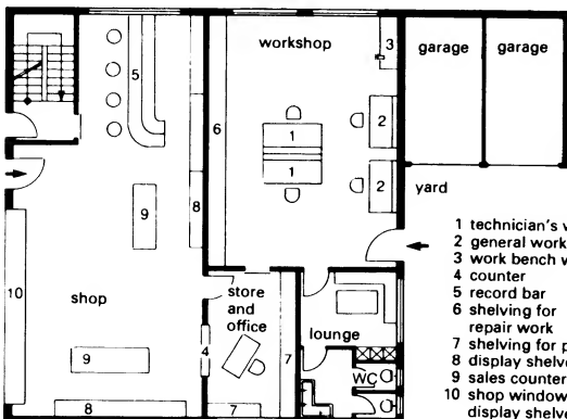
③ Example of an electrical repair (ground floor)
